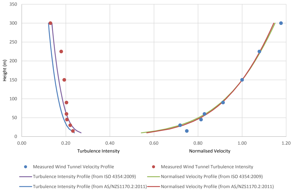
Mean Velocity and Turbulence Intensity for Suburban/Forest Terrain ( 0.2\text{m} < z_0 < 0.3\text{m} ) (TC3) at a 1:300 Scale
