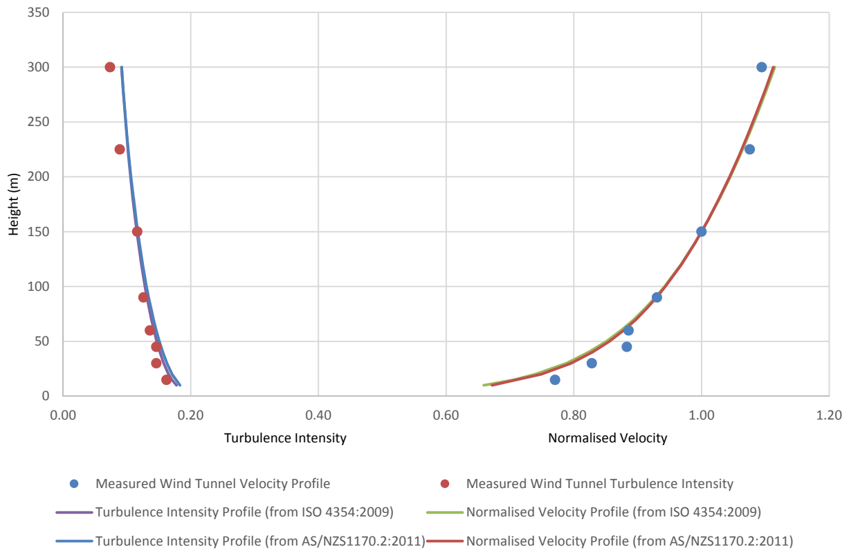
Mean Velocity and Turbulence Intensity for Open Terrain ( 0.02\text{m} < z_0 < 0.03\text{m} ) (TC2) at a 1:300 Scale
